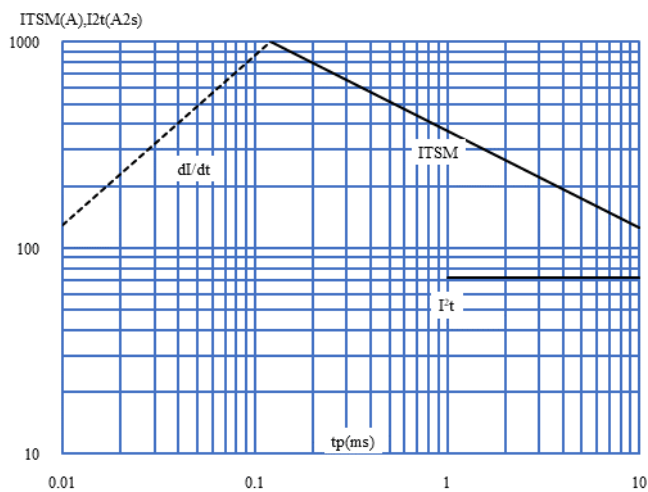
FIG.5: Non-repetitive surge peak on-state current for a sinusoidal pulse with width t_p < 20\text{ms} , and corresponding value of I^2t ( I -II-III: dI/dt < 50\text{A}/\mu\text{s} ; IV: dI/dt < 10\text{A}/\mu\text{s} )
